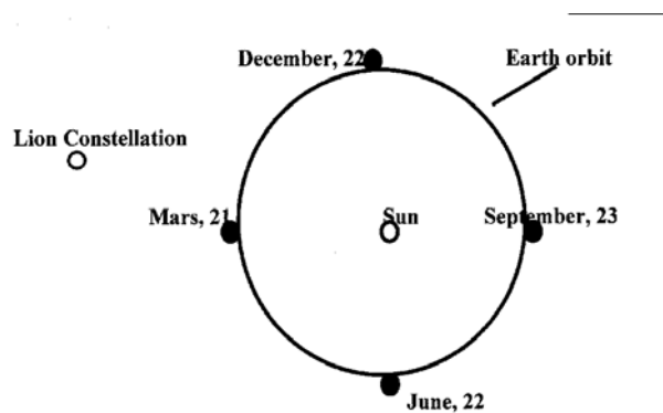
Figure 4. The Sun and Lion constellation disposition relative to Earth
